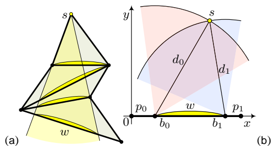
Figure 2: (a) Pencil of rays from the source vertex s passing through window w over the strip of unfolded triangles. (b) The position of the source v_s (or more generally pseudosource s ) is parameterized relative to the window w that lies on edge \overline{p_0p_1} .
